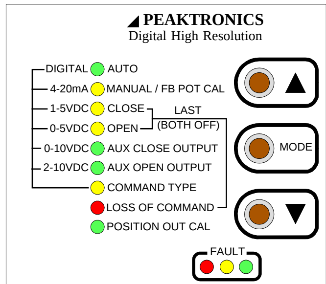
Figure 2 - Control Panel DHC-100x/200x Gen2 DHC-301 DHC-400
