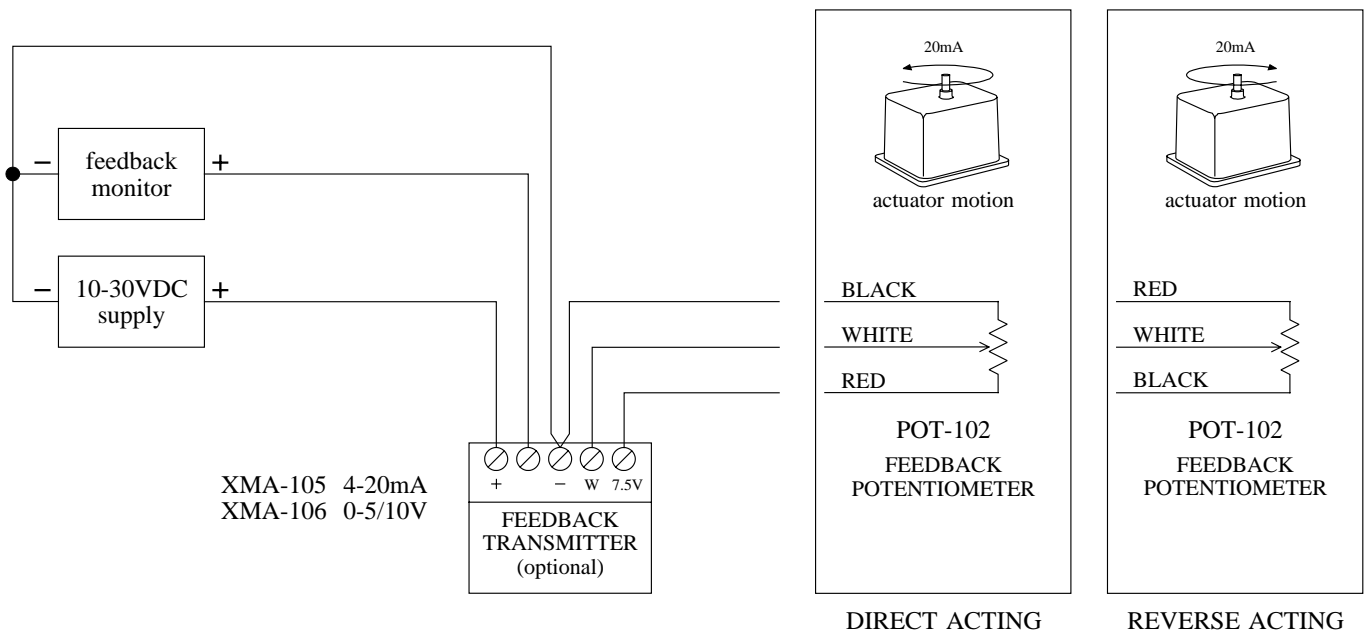
Wiring Diagram for Tyco actuator EPI Lite
