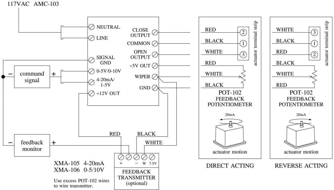
Wiring Diagram for Tyco actuator EPI Lite
